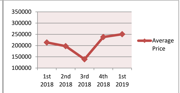
Last 5 Quarters
